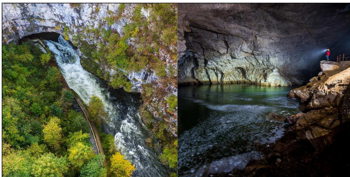
Figure 2.09: Planinska Jama. Left: Cave entrance. Right: Confluence of the Pivka and Rak Branches (Photos: M. Blatnik; RI-SI-EPOS).
