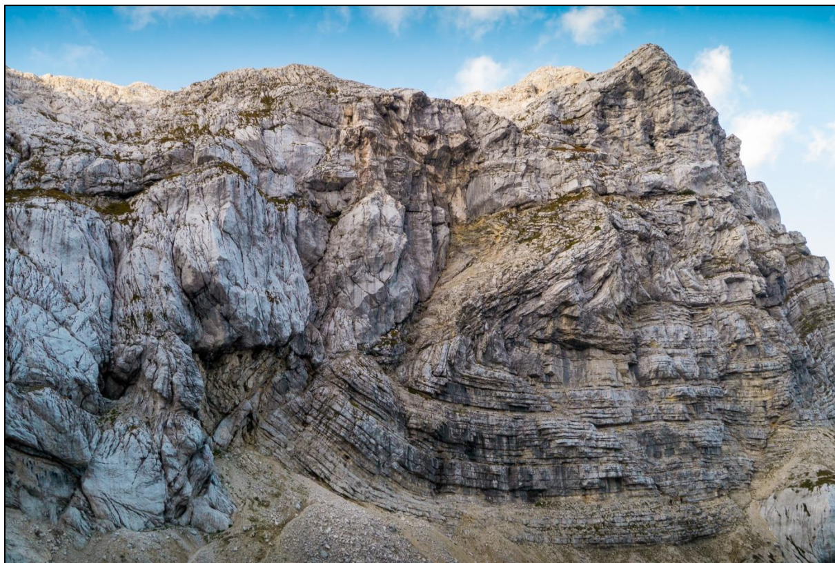
Figure 4.02: A contact between two different formations at Kanjavec Mountain (Photo: M. Blatnik).
